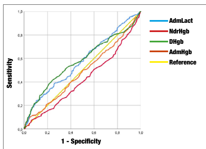
Figure 1. Receiving operating characteristic (ROC) curves for assessing the predictive accuracy of AdmHgb, MaxHgb, NdrHgb, DHgb and admission lactate for mortality
